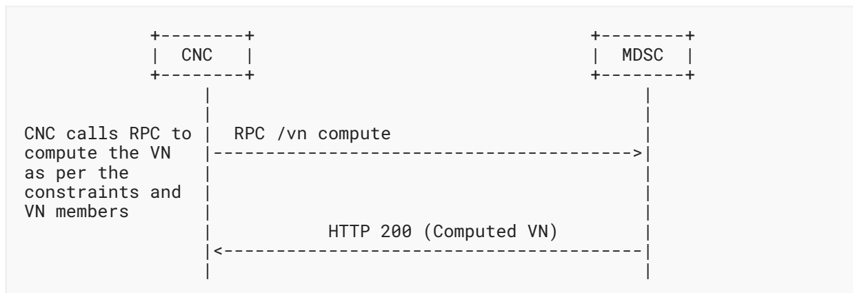
Figure 10: VN Compute
