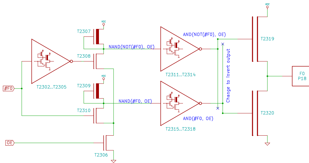
Figure 4.24: Schematic of the output stage
