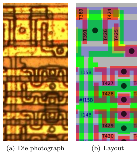
Figure 4.15: A part of the product term array
