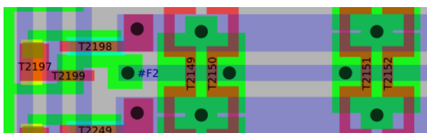
Figure 4.20: Layout of a part of the sum term array
