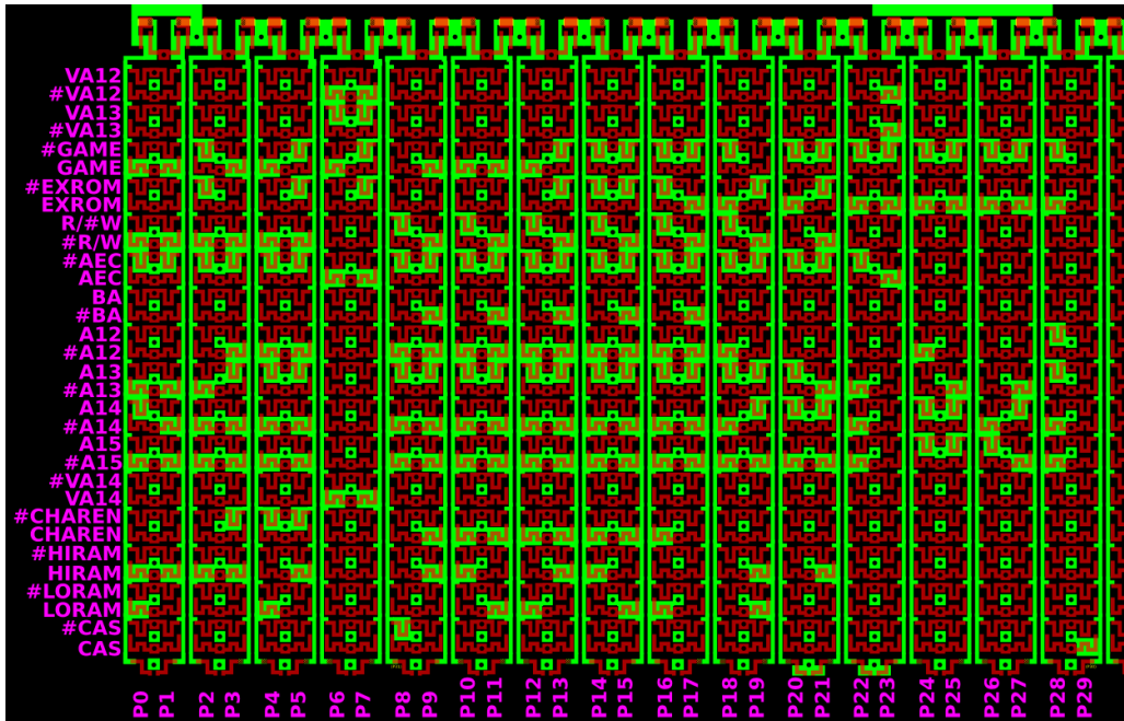
Figure 4.14: Product terms made readable in the layout
