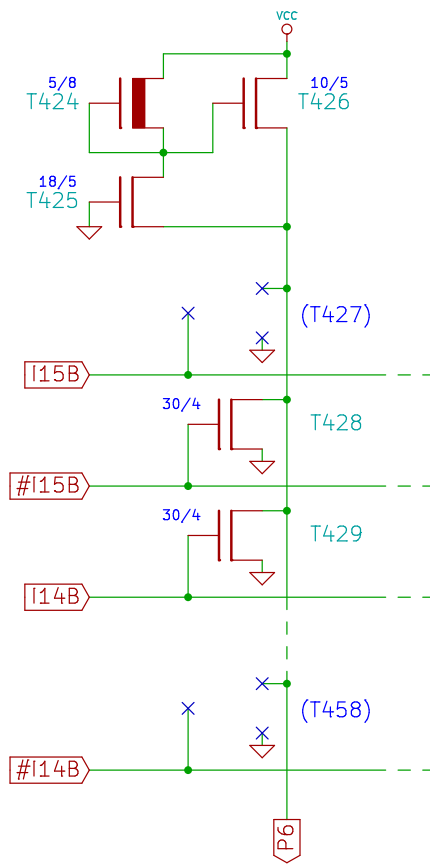
Figure 4.16: Schematic of a part of the product term array
